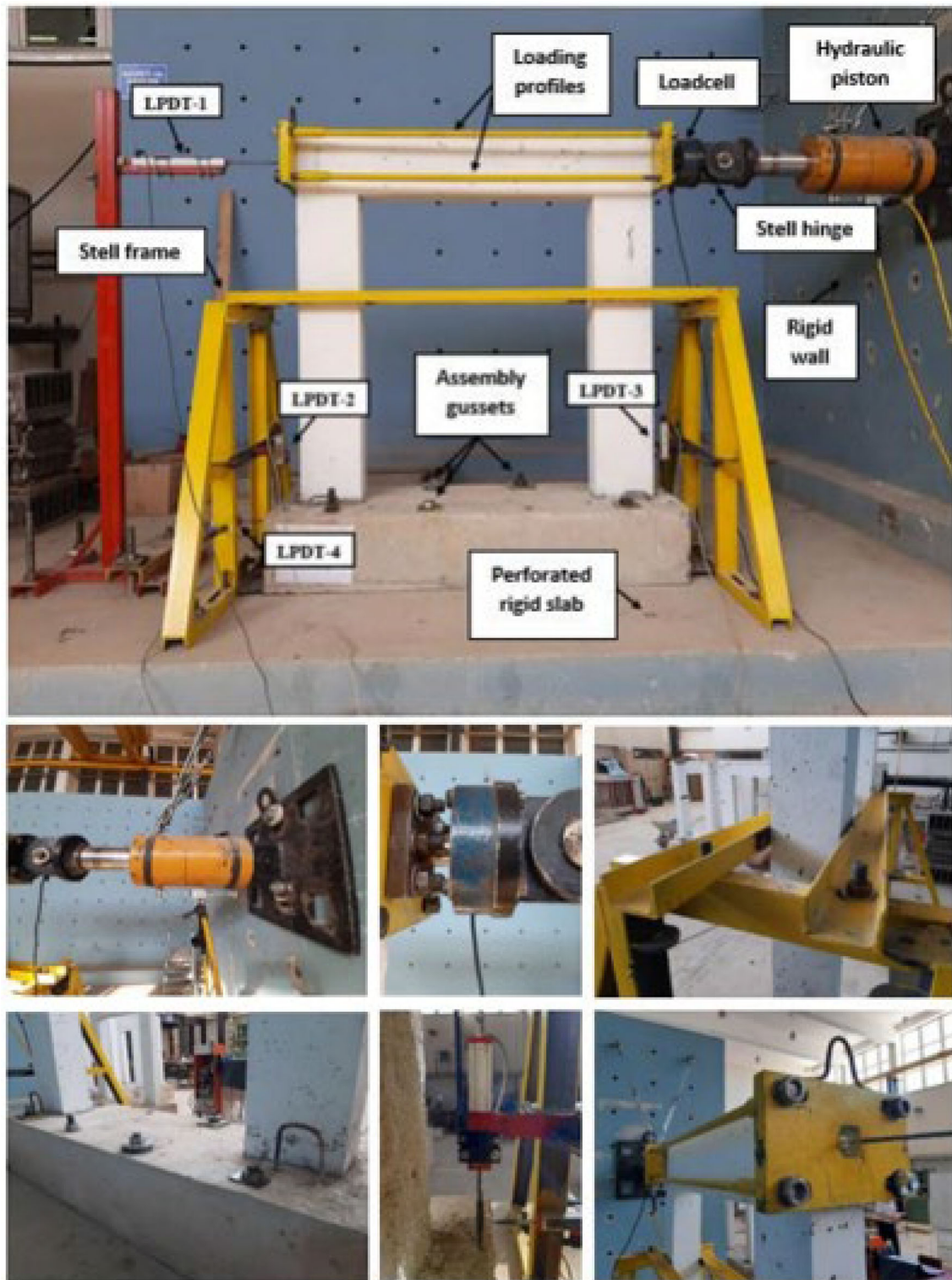
Fig. 5 Application of cyclic lateral load
