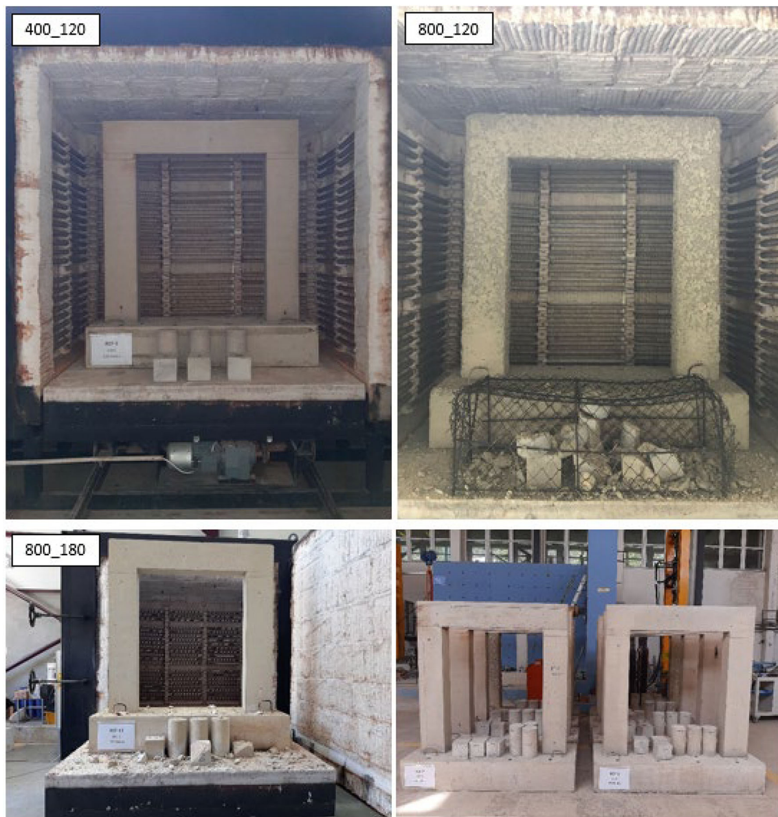
Fig. 4 Concrete specimens subjected to high-temperature effect
