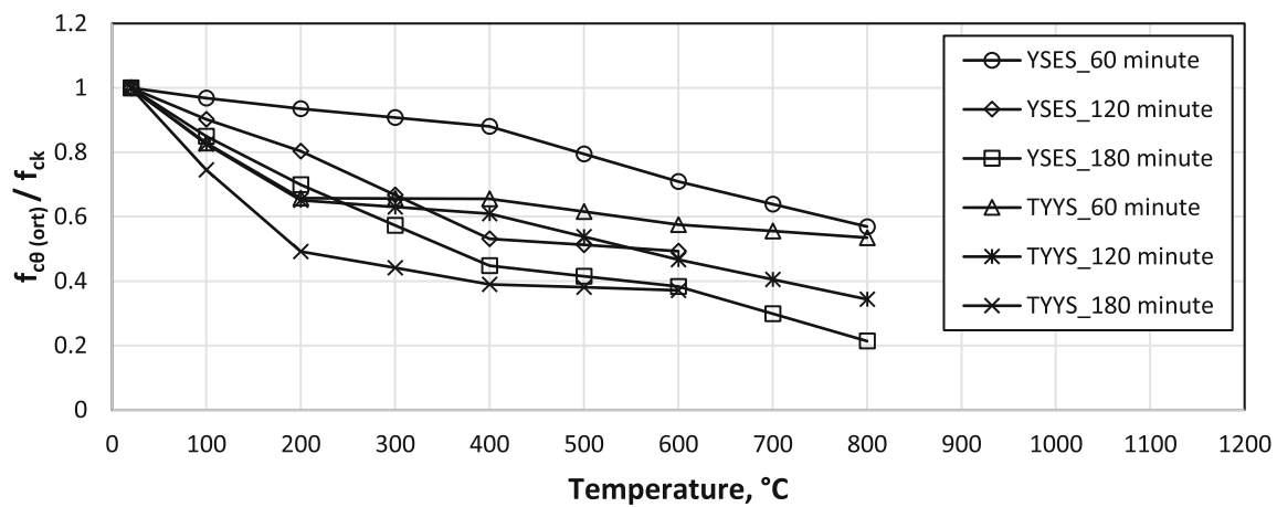
Fig. 9 Variation of compressive strength with temperature. f_{ck} ; Compressive strength of reference standard cylinder concrete specimen not exposed to high temperature
