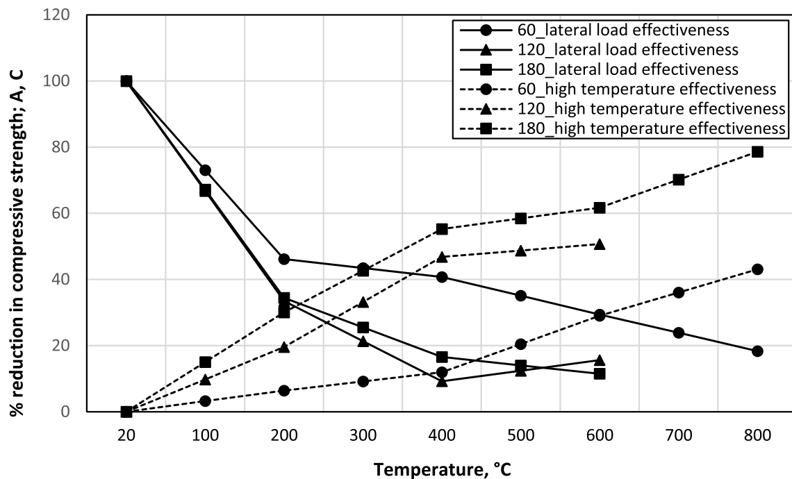
Fig. 10 Variation of the effectiveness of lateral load and high temperature on the decrease in compressive strength with temperature
