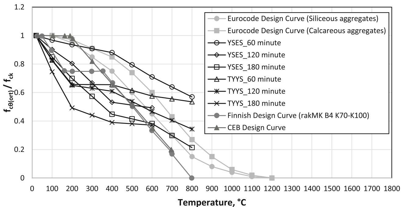
Fig. 11 Comparison of design curves and experimental strength loss curves
