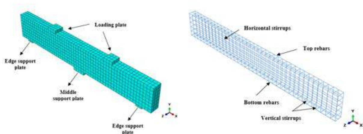
Figure 6. Finite element model of deep beam without openings (RCDB-R)
