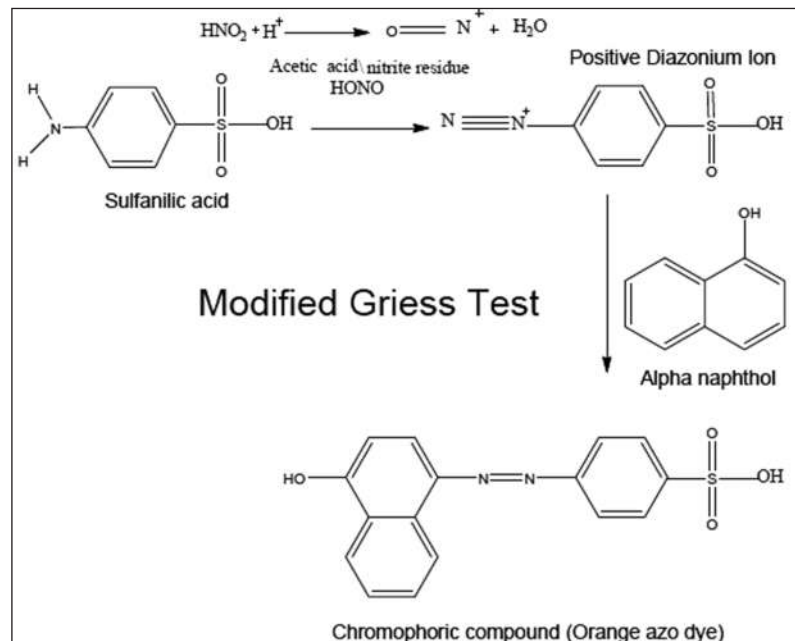
FIGURE 1: The chemical reaction for the Modified Griess Test (The orange color is caused when the nitrites are introduced to acetic acid and heated to form nitrous acid. The nitrous acid then forms a diazonium compound with sulfanilic acid, and this compound then couples with the alpha-naphthol to produce the orange azo dye).
