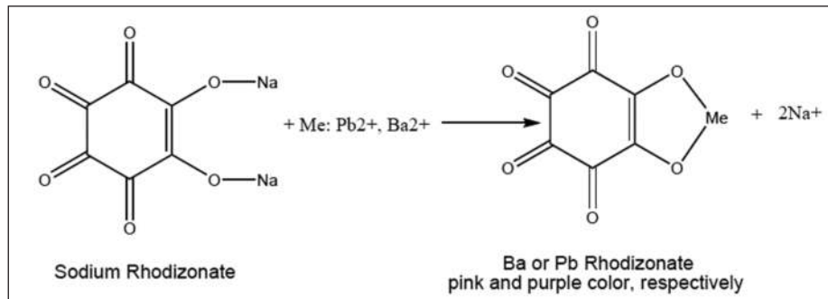
FIGURE 2: The chemical reaction describing the Sodium Rhodizonate Test.
