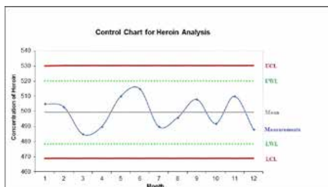
Figure 4. Control chart of heroin, performed by GC-FID. Concentration of heroin is given in \mu\text{g/mL} while UCL, UWL, LWL and LCL stand for upper control limit, upper warning limit, lowest warning limit and lowest control limit, respectively. The blue line represents the stability in the heroine concentrations measured over months.
